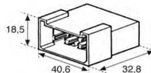
• 8-way male
