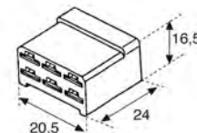
• 6 way female
