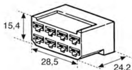
• 8 way female
