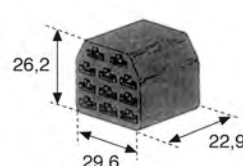
• 11 way female
