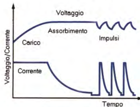
Diagramma di carica XS 3600
